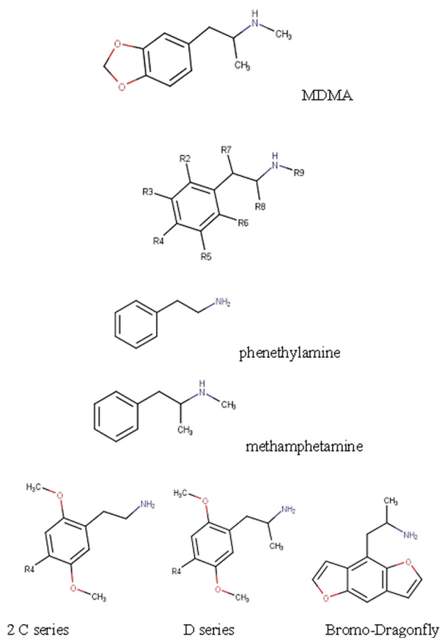
Figure 1: Chemical structures of some members of the phenethylamines family of drugs [296]. Reprinted from Drug and Alcohol Dependence, 154, Gael Le Roux, Chloe Bruneau, Benedicte Lelievre, Marie Bretaudeau Deguigne, Alain Turcant, Patrick Harry, David Boels, Recreational phenethylamine poisonings reported to a French poison control center, 46–53, 2015, with permission from Elsevier.
